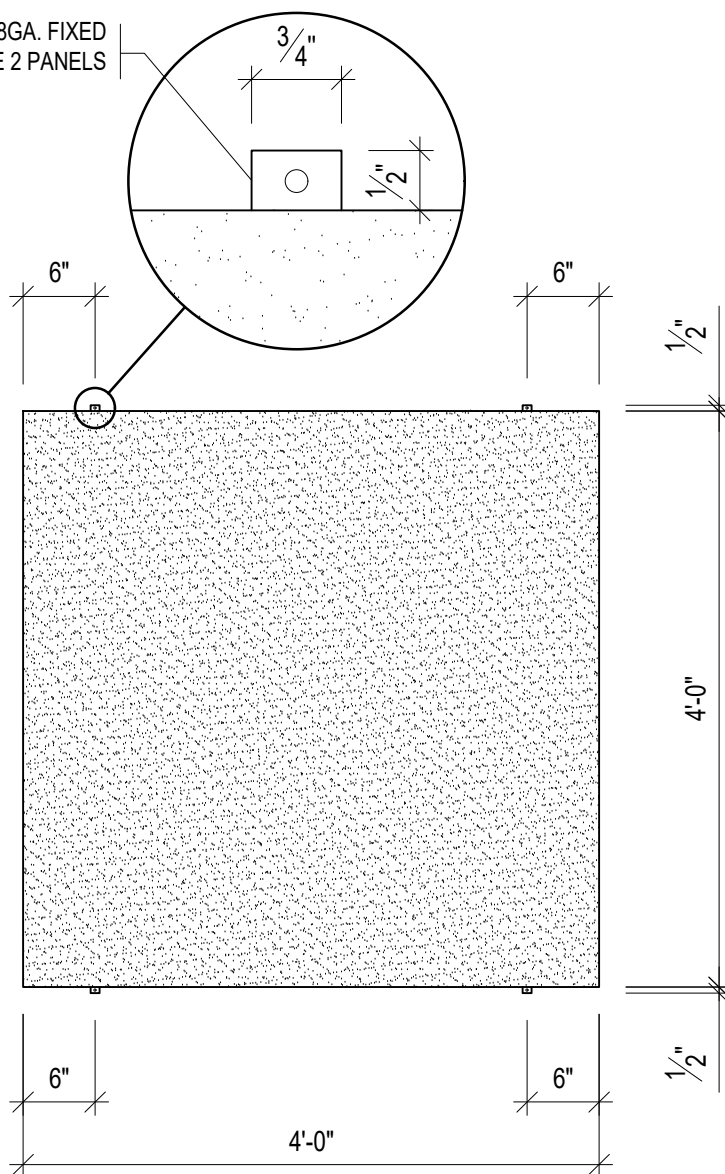
FRONT VIEW
