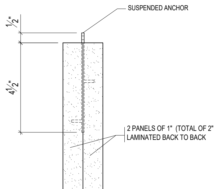
ANCHOR DETAIL SIDE VIEW
