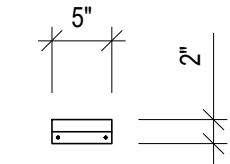
FRONT VIEW WALL ANCHOR
