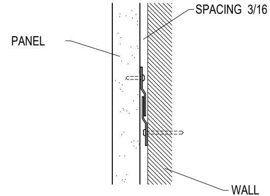
WALL ANCHORING DETAILS
