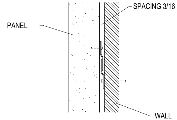
WALL ANCHORING DETAIL
