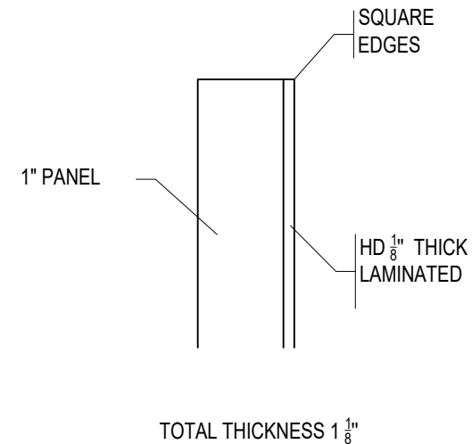
SIDE PANEL DETAIL WITH NO FABRIC
