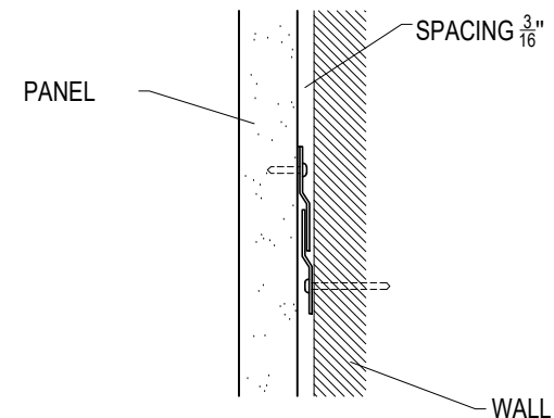
WALL ANCHORING DETAL
